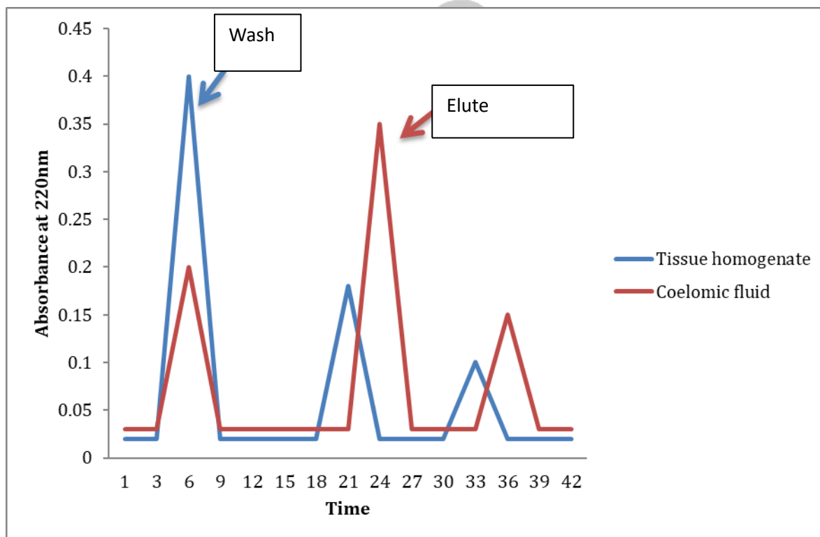
Fig.1: Anion exchange chromatography.
