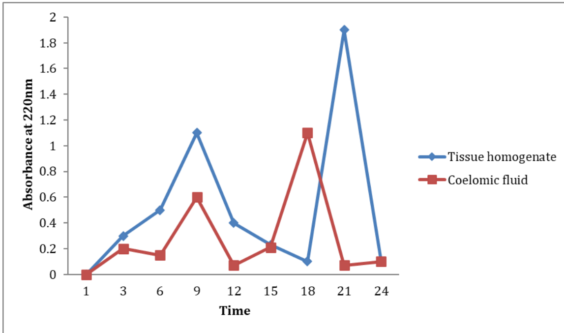
Fig.2: Gel filtration chromatography.
